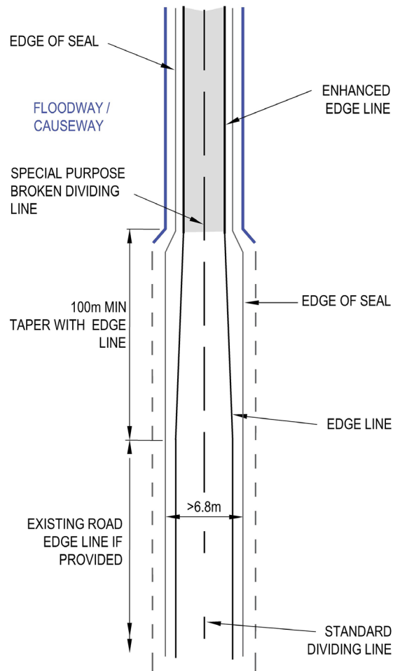
NARROWING OF ROAD FORMATION AND / OR SEAL WIDTH
