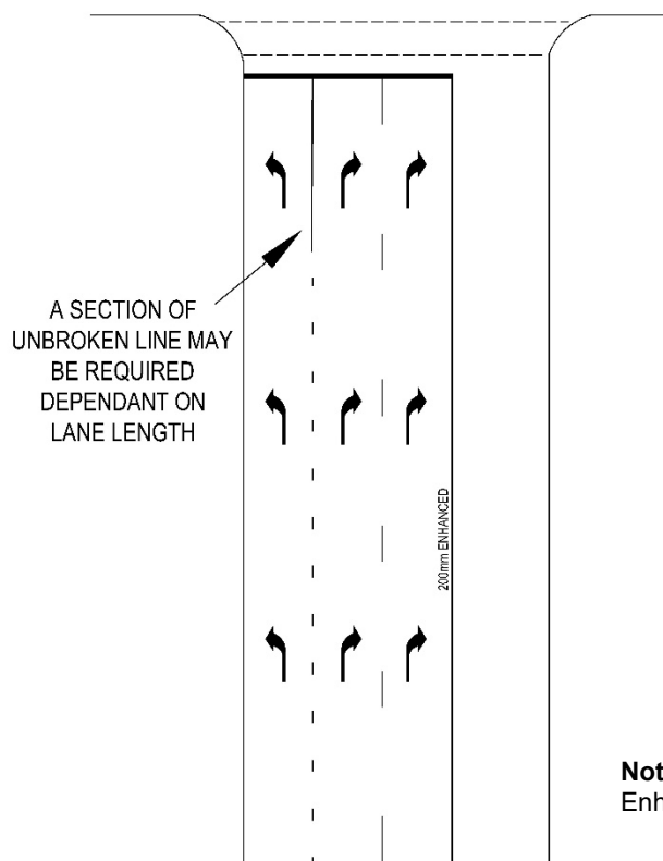
3 ROWS WHERE LENGTH PERMITS
