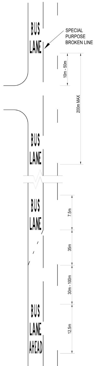
PART-TIME BUS LANE
