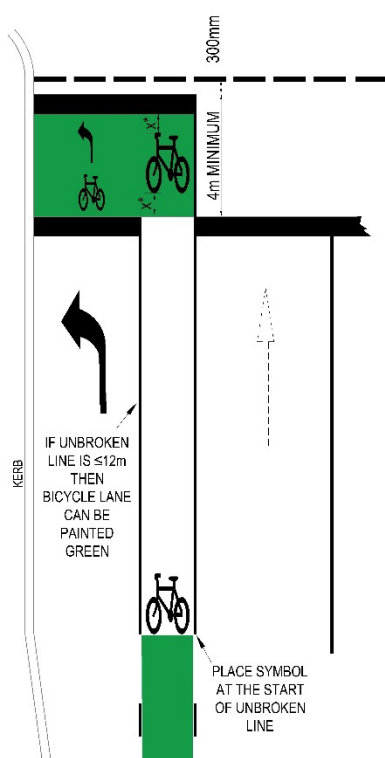
WITH A BICYCLE LANE
