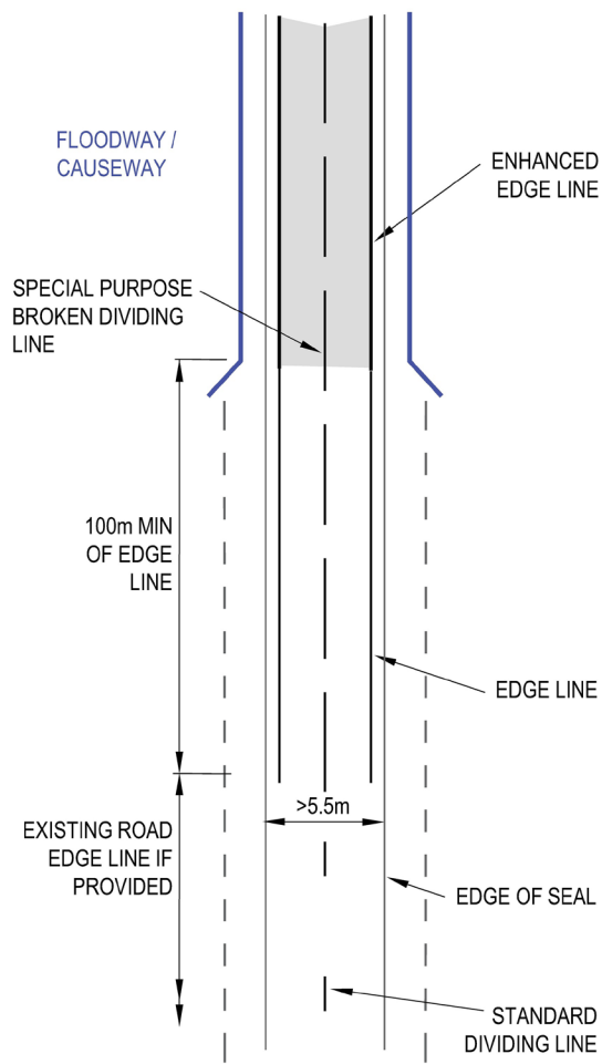
NO NARROWING OF ROAD FORMATION OR SEAL WIDTH
