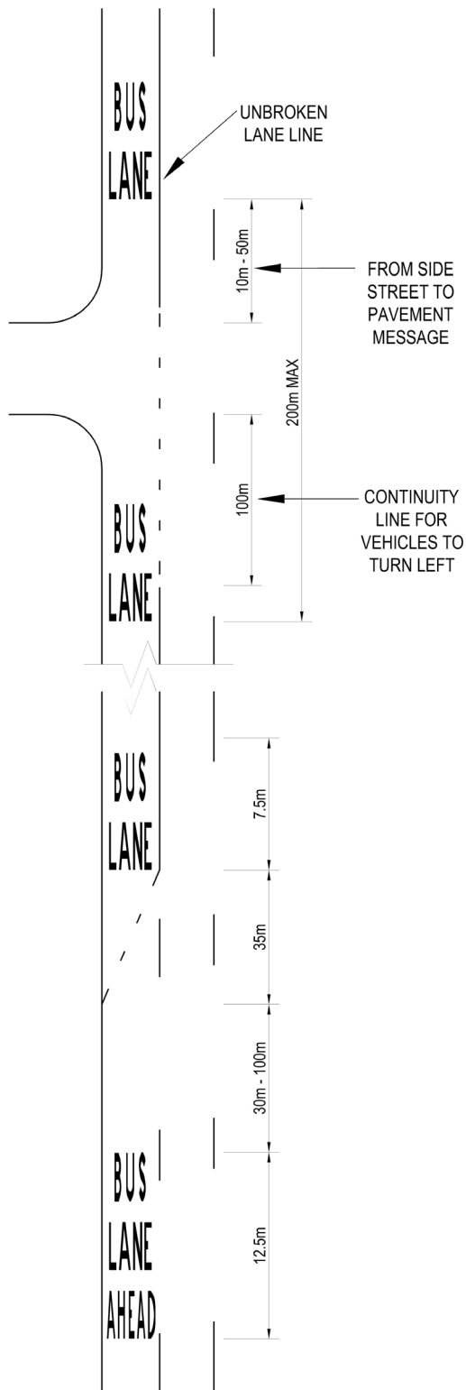
FULL TIME BUS LANE
