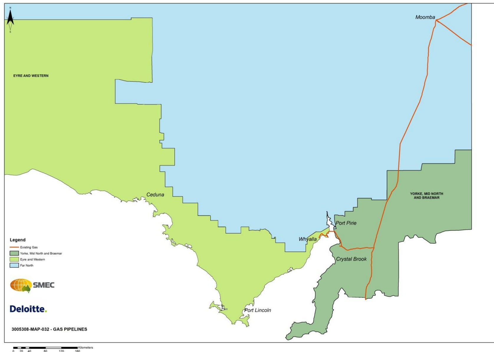
Figure 5.5: Overview of the existing gas network impacting the Eyre and Western region
