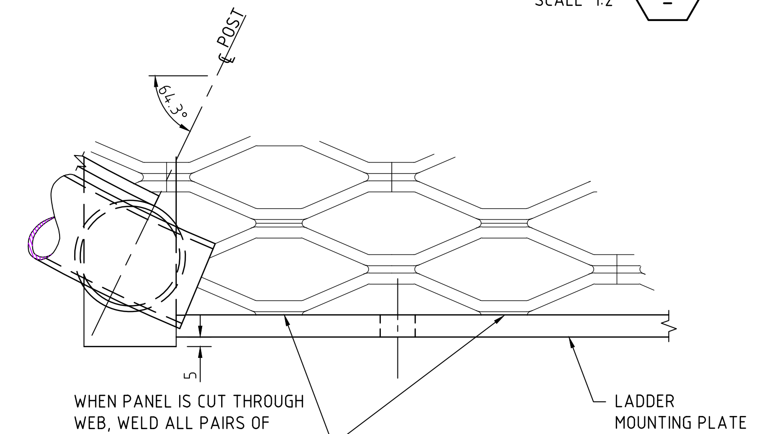
DETAIL C SCALE 1:2
