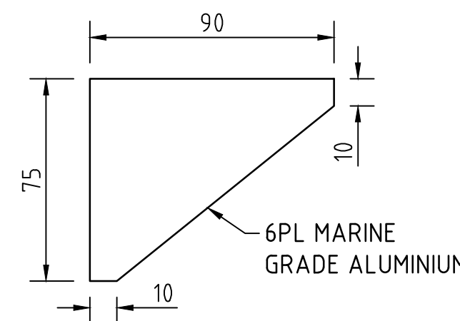
GUSSET PLATE SCALE 1:2
