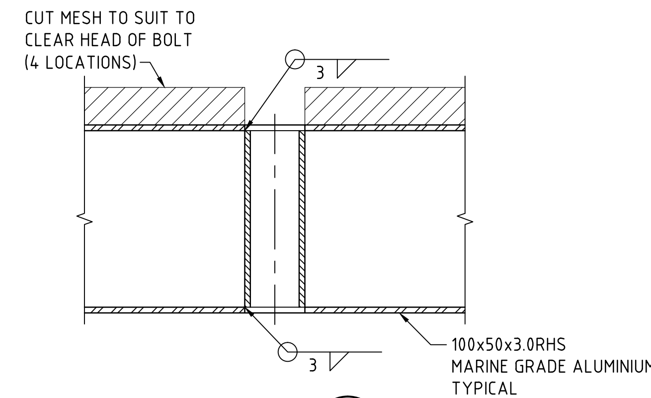
SECTION 1 SCALE 1:2
