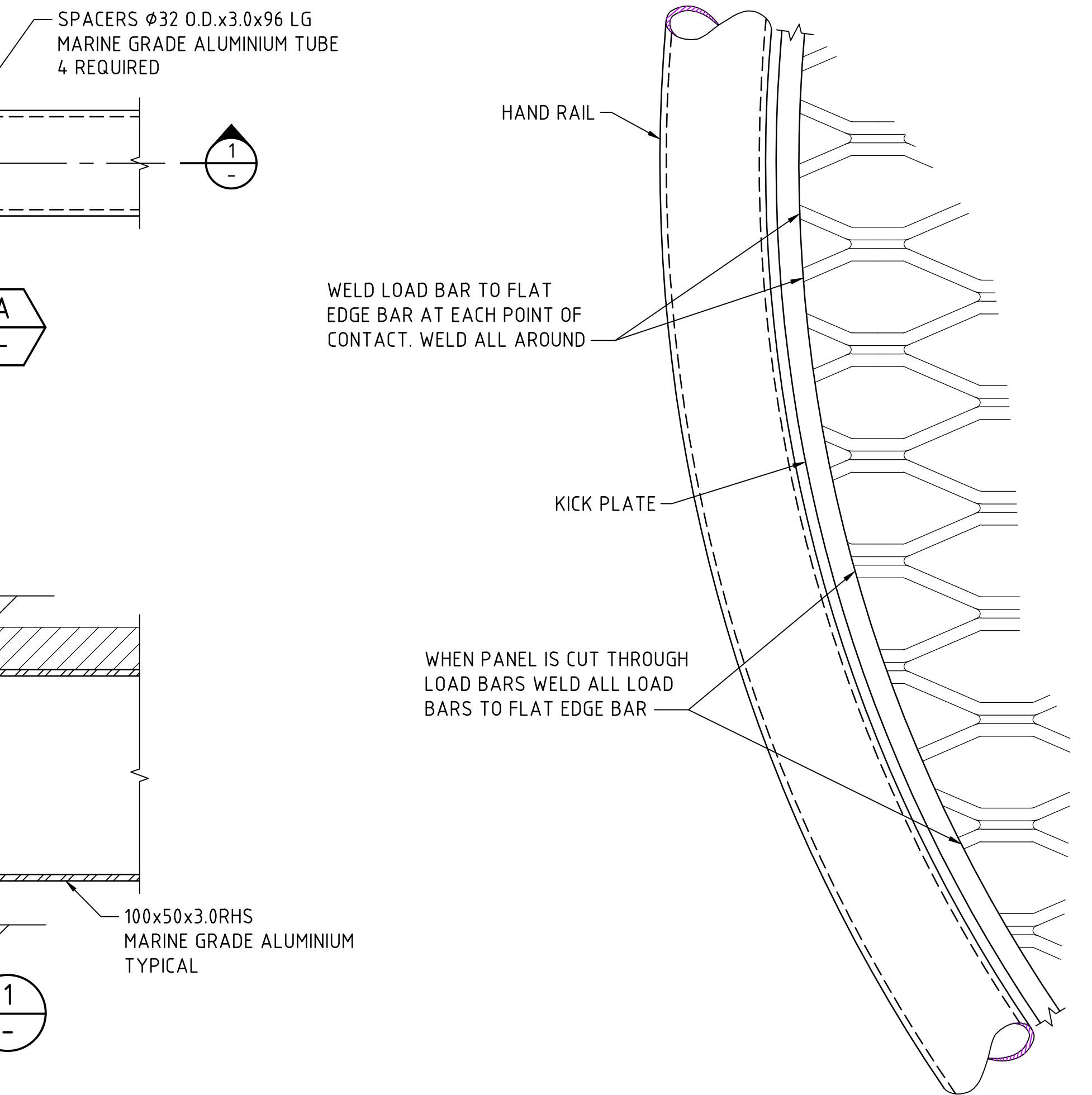
DETAIL B SCALE 1:2
