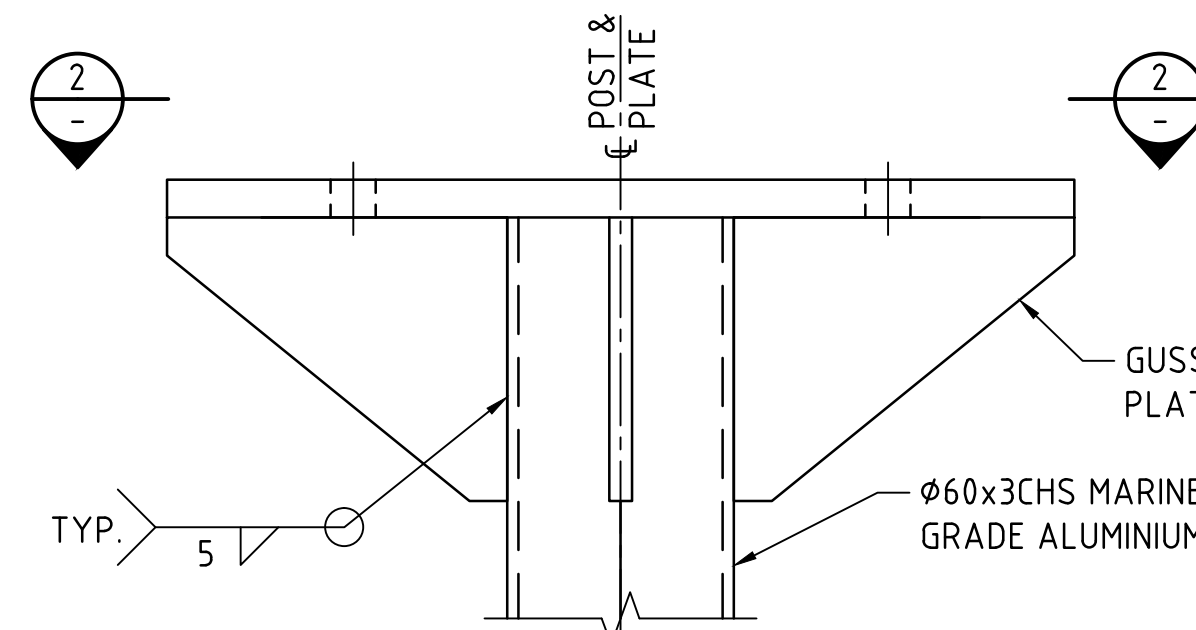
DETAIL D SCALE 1:2
